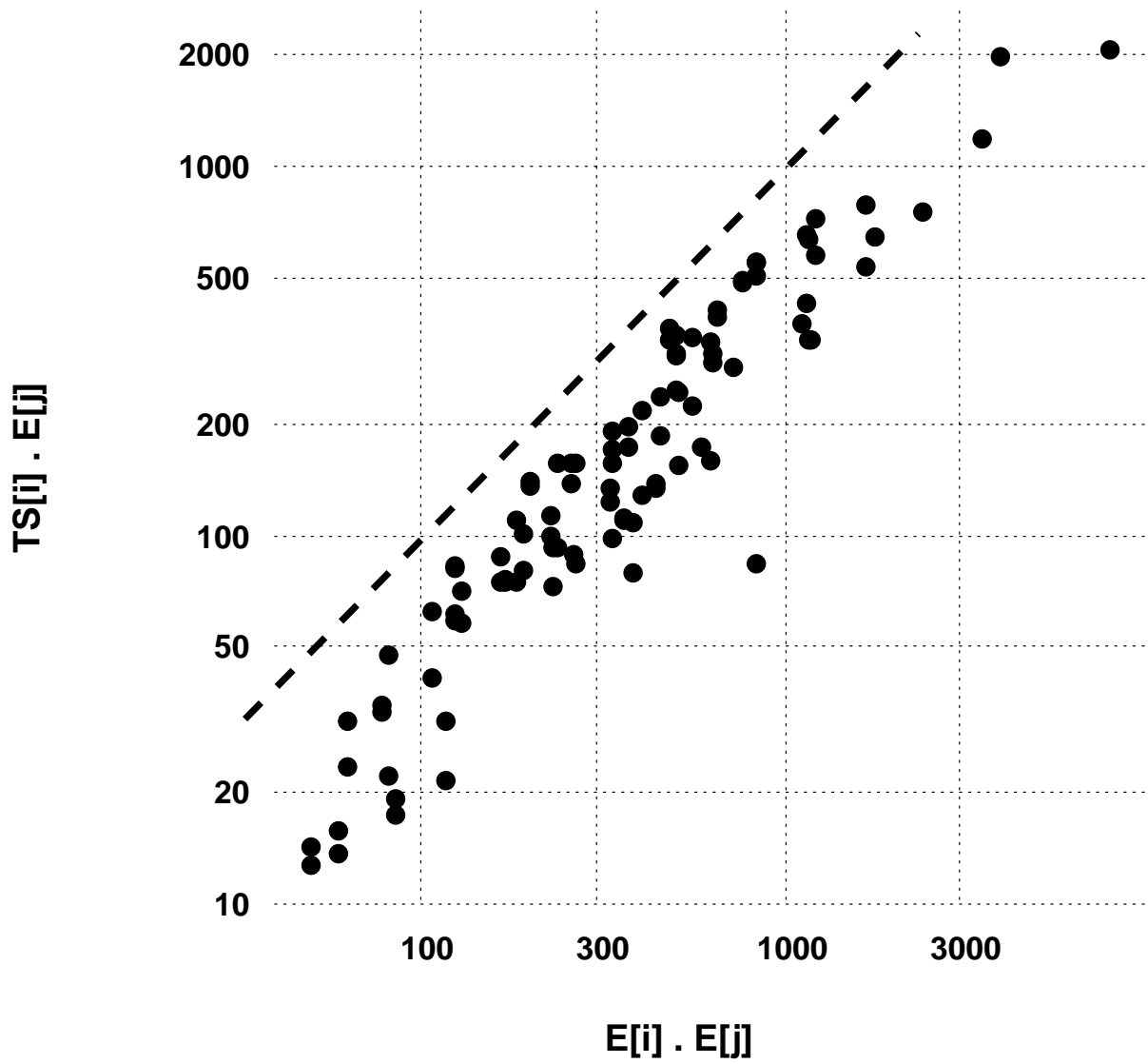
Fig. 1 English scores vs Translated Spanish scores
